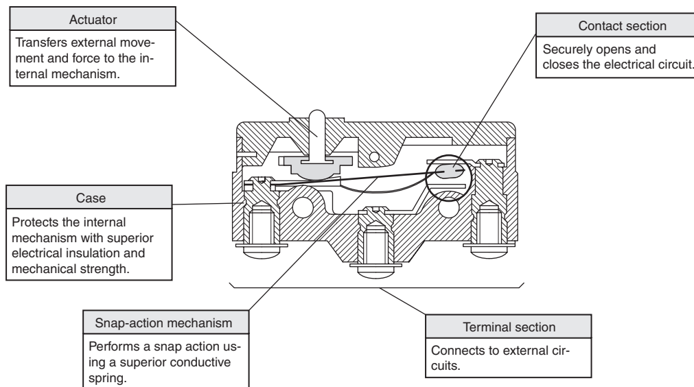
Structural Diagram of Typical Basic Switch
