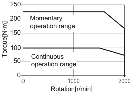
• R88M-1M15K015C
