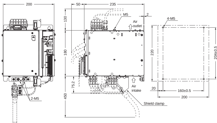
Mounting dimensions
