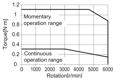
• R88M-1M10030T
