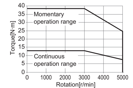
• R88M-1L4K030C
