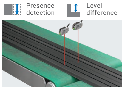
Presence detection of tires
