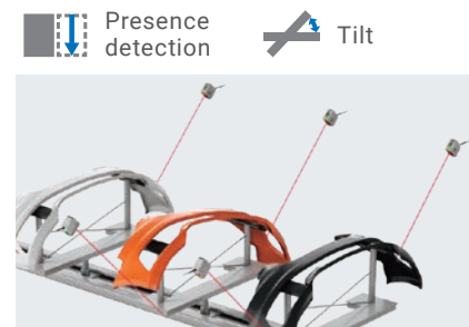
Bumper presence and tilt detection
