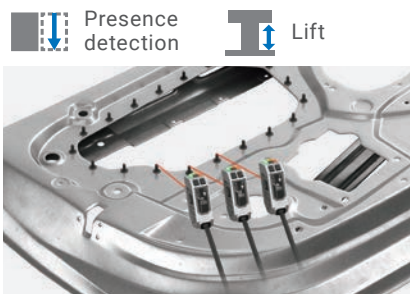
Presence detection of door parts
