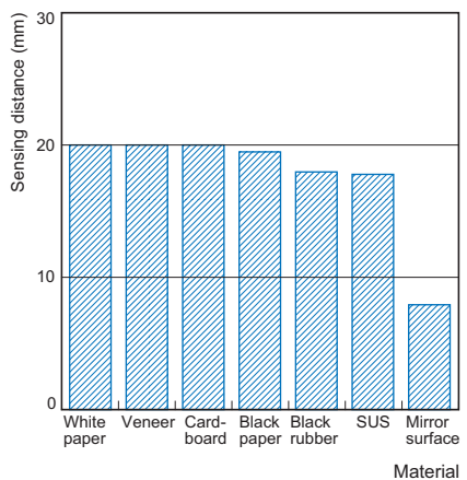
Set Distance of 20 mm using White Paper
