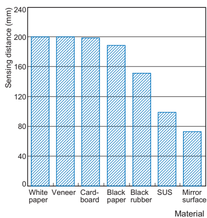
Set Distance of 200 mm using White Paper
