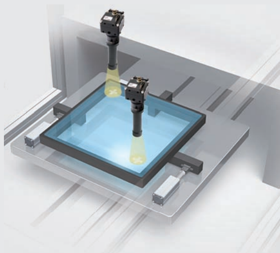
Illustration of Alignment Mark Detection
