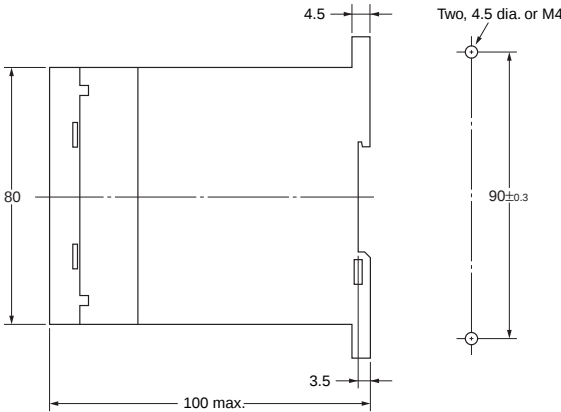
Mounting Holes
