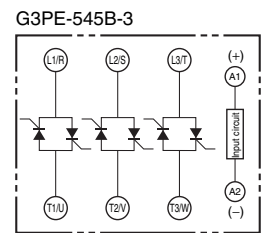
Terminal Arrangement/Internal Circuit Diagram
