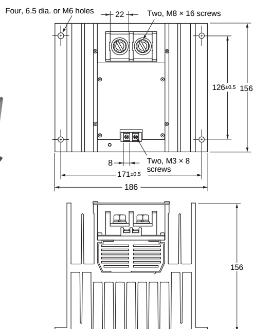
Mounting Hole Dimensions
