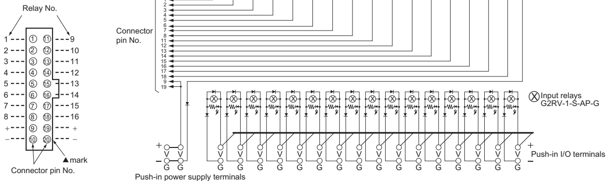
Connector Pin (male) Configuration View from engaged side
