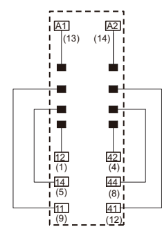
Terminal Arrangement/Internal Connection Diagram (Top View)
