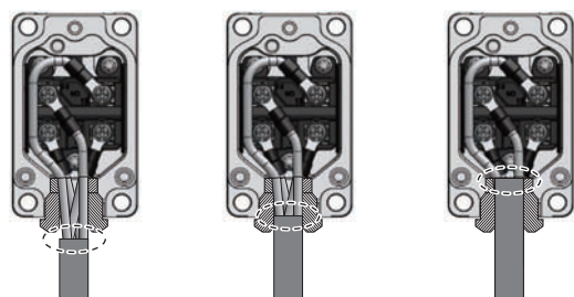
(1) Connector tube contains internal stranded wire
