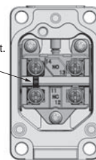
Terminal Plate Mounting Diagram
