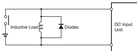
Diagram 6. Input Signal Noise Countermeasures
