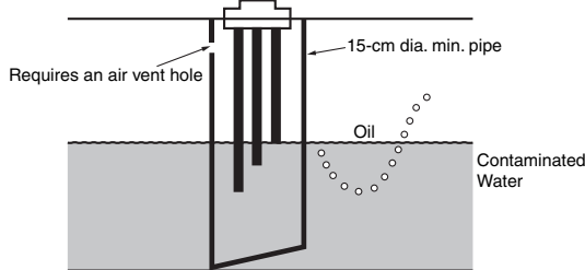
Cut off the end of the pipe at an angle to keep the oil from the electrodes.
