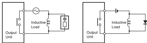
Diagram 7. Output Signal Noise Countermeasures
