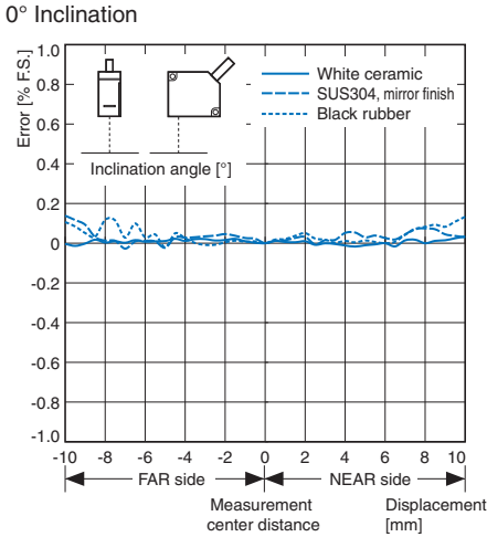
Example: Characteristic of the ZX2-LD50
