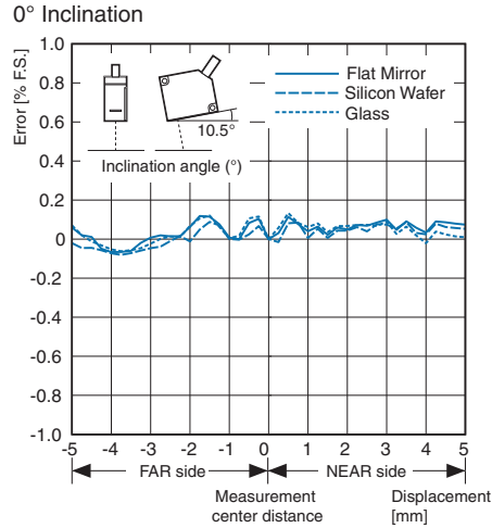
Example: Characteristic of the ZX2-LD50V
