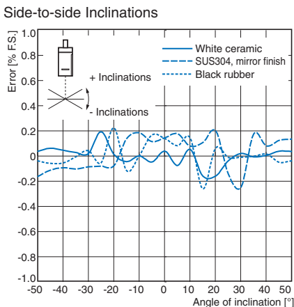
Example: Characteristic of the ZX2-LD50
