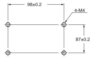
Mounting screw holes
